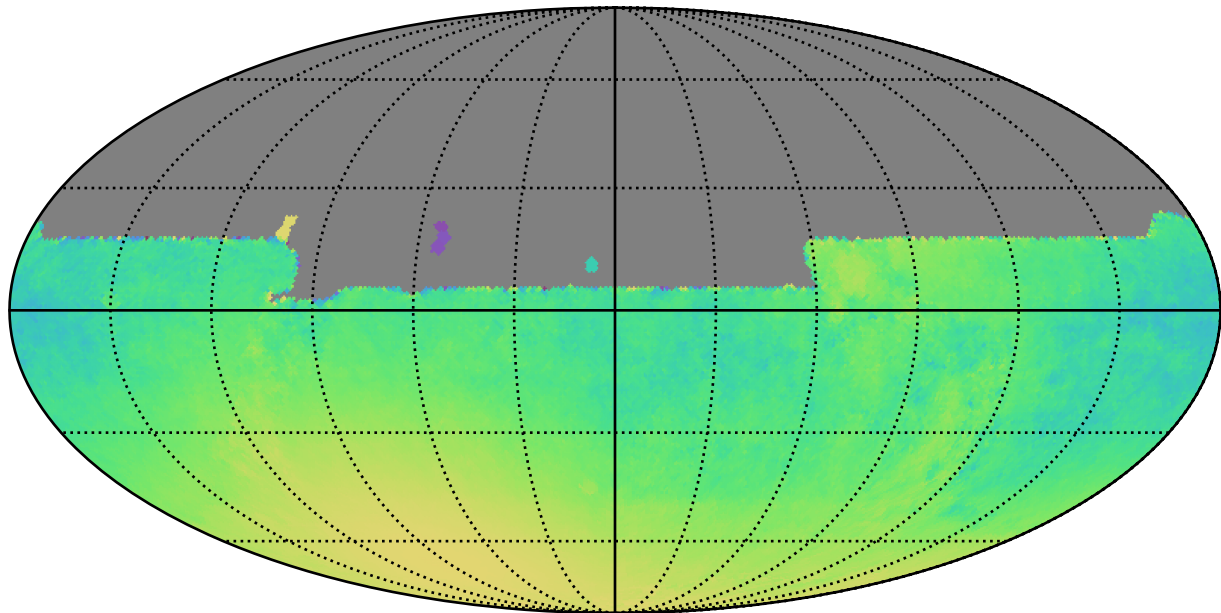
too_combined_no_nss_s10.0_v3.4_10yrs All sky y band only: Normalized Parallax Uncert @ 21.3
