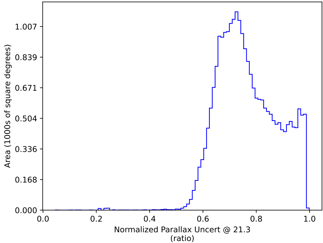
too_combined_no_nss_s10.0_v3.4_10yrs All sky y band only: Normalized Parallax Uncert @ 21.3
