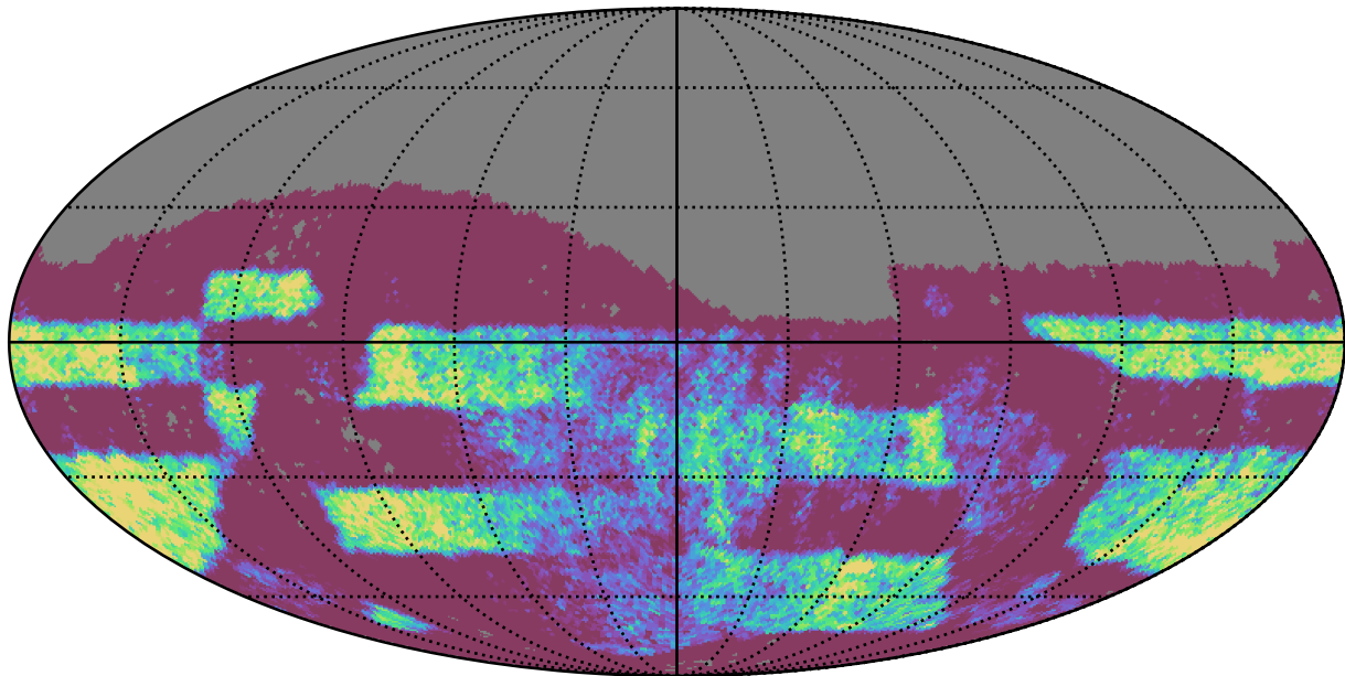
too_combined_no_nss_s10.0_v3.4_10yrs Yr 3-4 z band: NVisits
