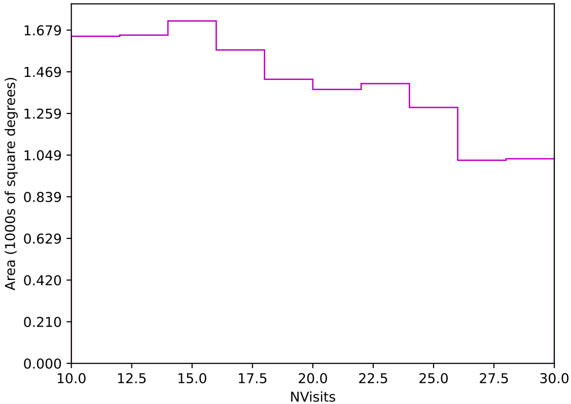
too_combined_no_nss_s10.0_v3.4_10yrs Yr 3-4 z band: NVisits
