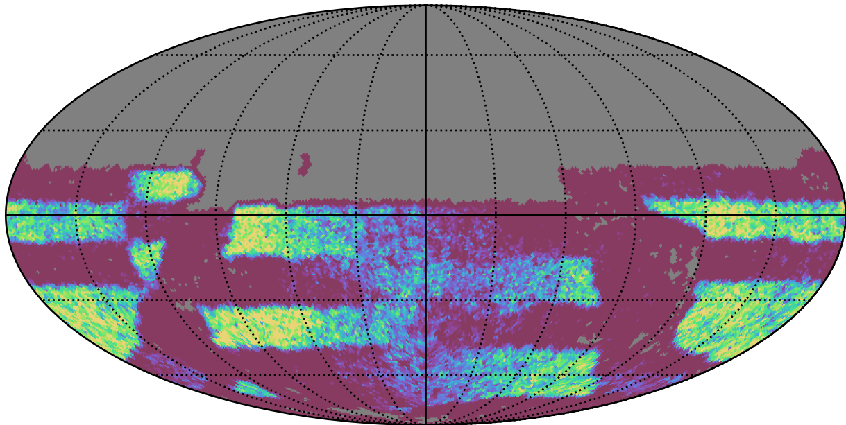
too_combined_no_nss_s10.0_v3.4_10yrs Yr 3-4 y band: NVisits
