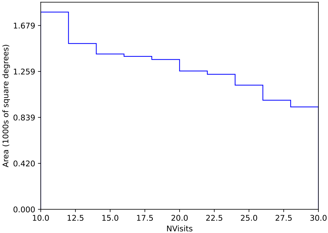
too_combined_no_nss_s10.0_v3.4_10yrs Yr 3-4 y band: NVisits
