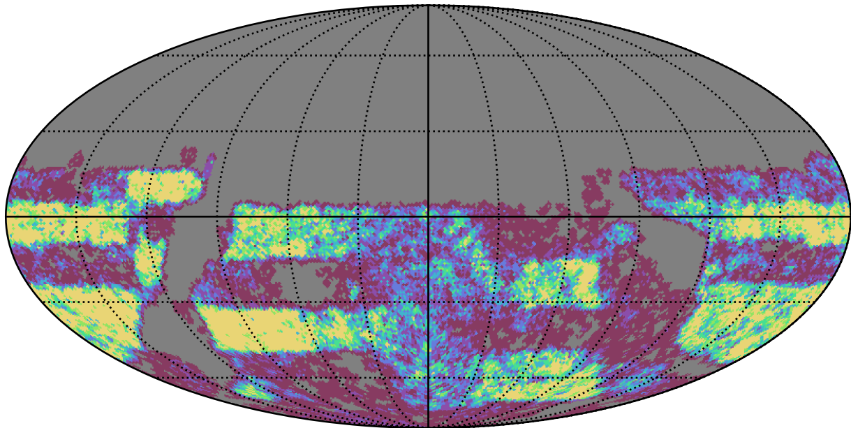
too_combined_no_nss_s10.0_v3.4_10yrs Yr 3-4 u band: NVisits
