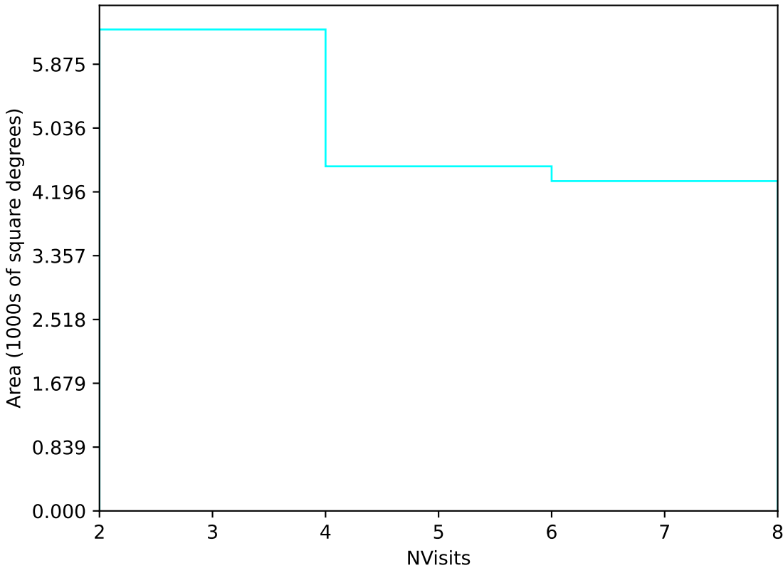
too_combined_no_nss_s10.0_v3.4_10yrs Yr 3-4 u band: NVisits
