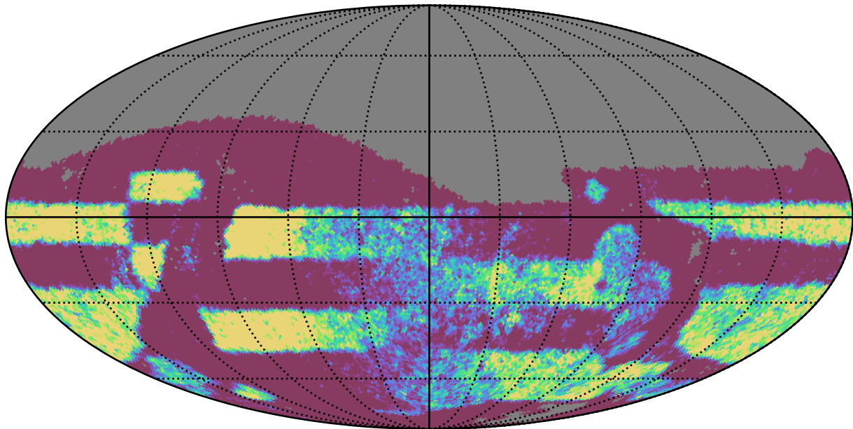
too_combined_no_nss_s10.0_v3.4_10yrs Yr 3-4 r band: NVisits
