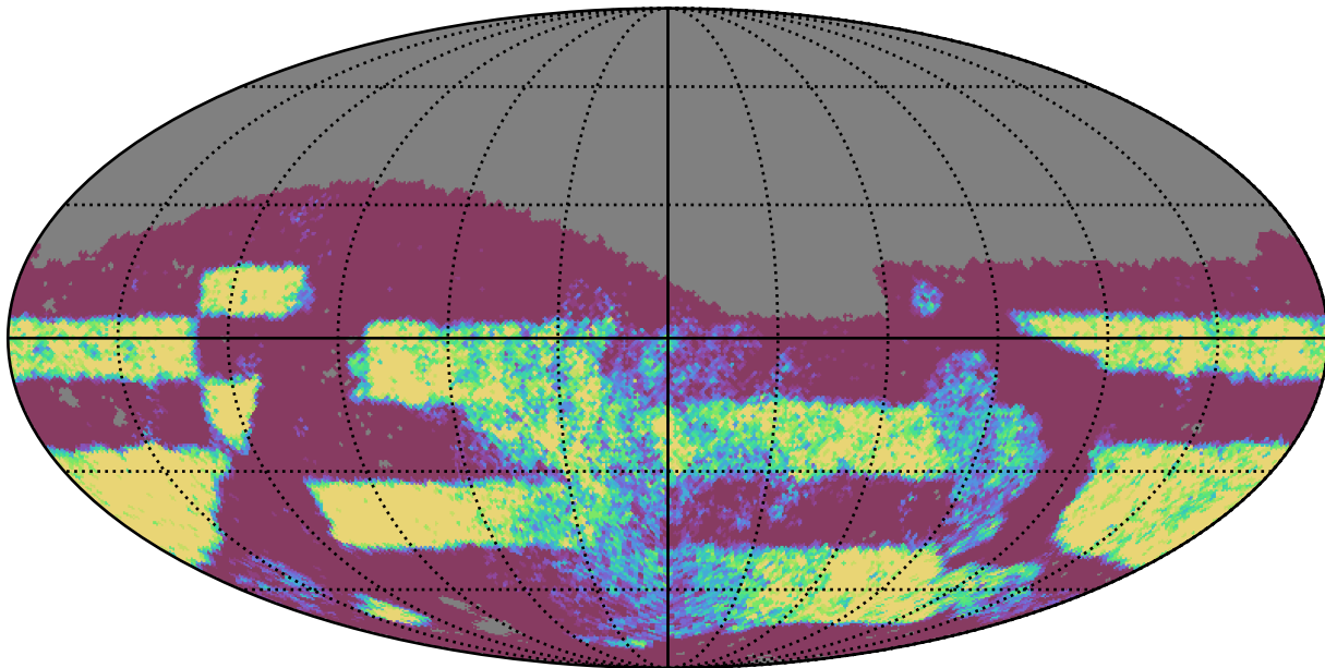
too_combined_no_nss_s10.0_v3.4_10yrs Yr 3-4 i band: NVisits
