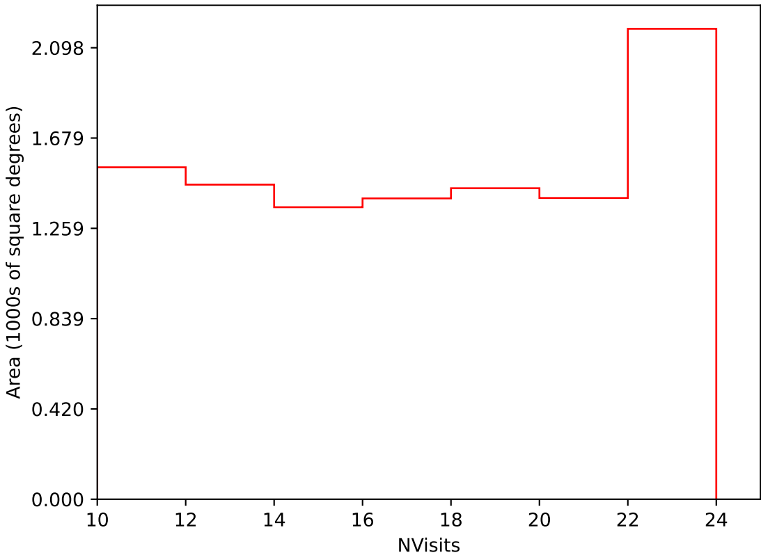
too_combined_no_nss_s10.0_v3.4_10yrs Yr 3-4 i band: NVisits
