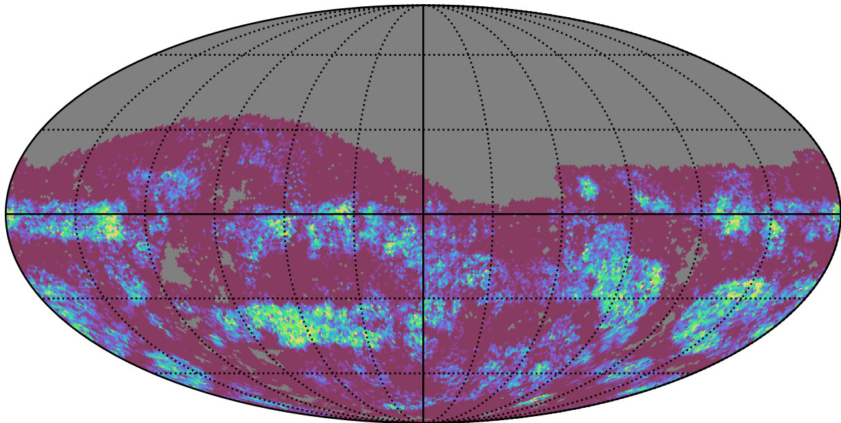
too_combined_no_nss_s10.0_v3.4_10yrs Yr 3-4 g band: NVisits
