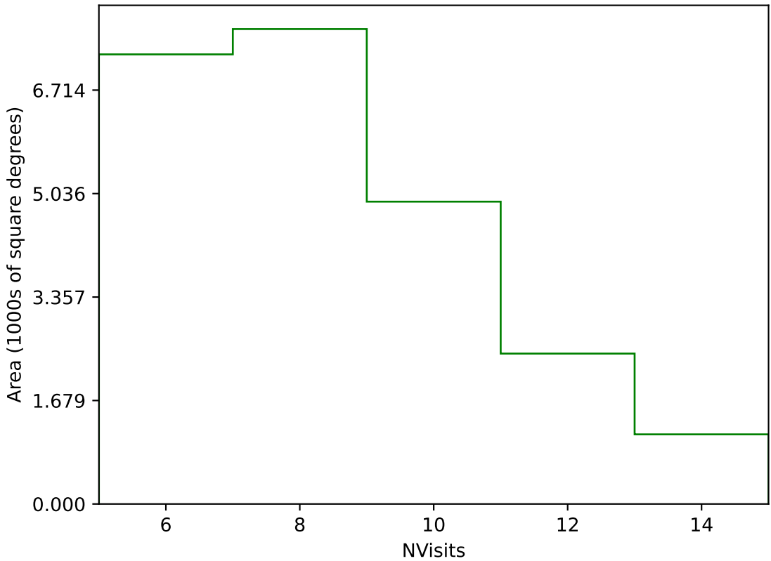
too_combined_no_nss_s10.0_v3.4_10yrs Yr 1 g band: NVisits
