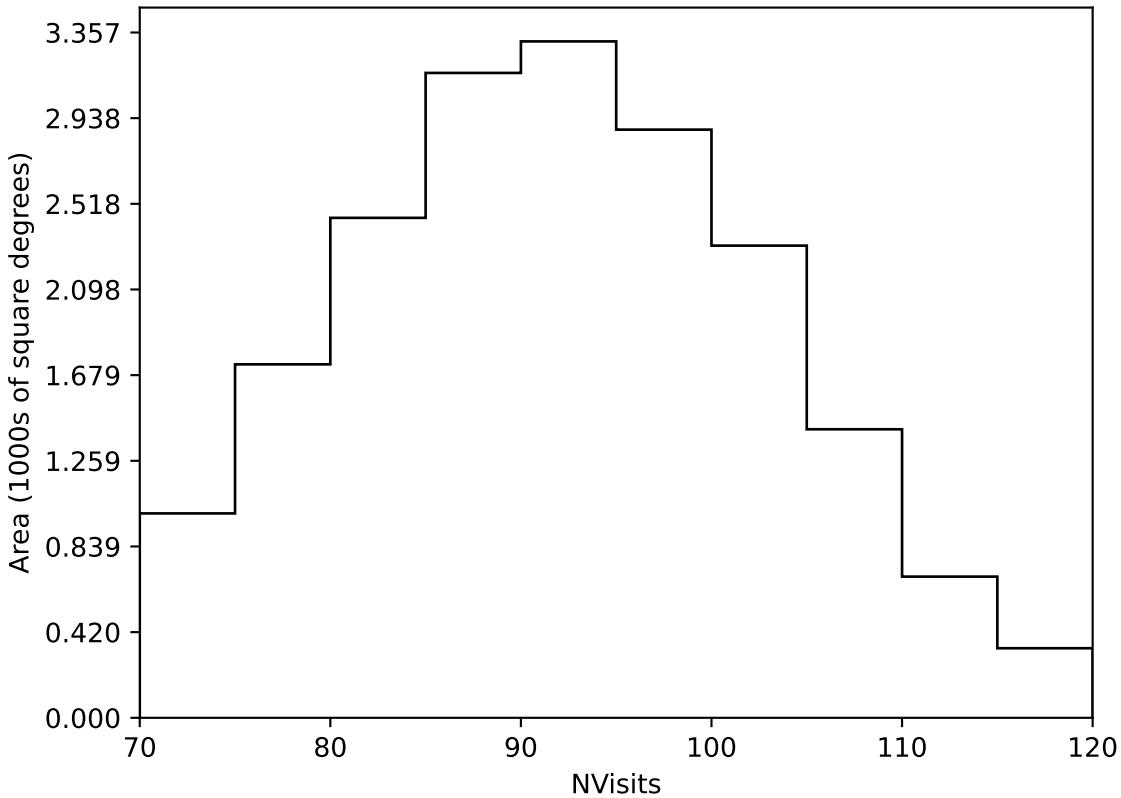
too_combined_no_nss_s10.0_v3.4_10yrs Yr 1 all bands: NVisits
