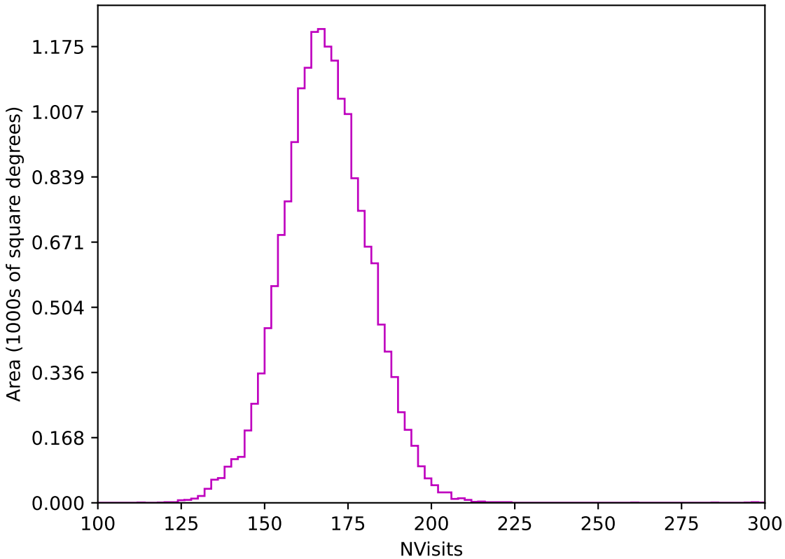
too_combined_no_nss_s10.0_v3.4_10yrs WFD z band: NVisits
