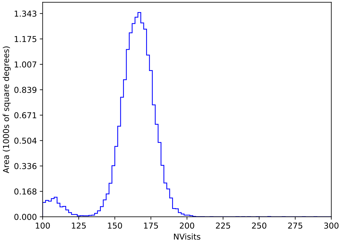
too_combined_no_nss_s10.0_v3.4_10yrs WFD y band: NVisits
