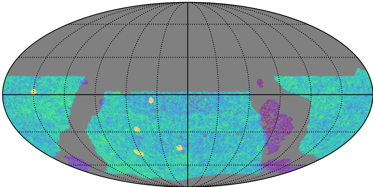
too_combined_no_nss_s10.0_v3.4_10yrs WFD u band: NVisits
