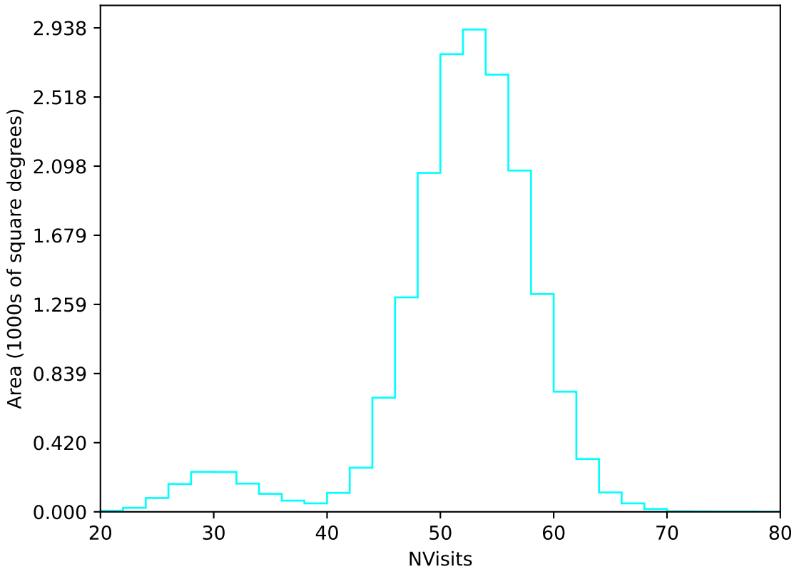
too_combined_no_nss_s10.0_v3.4_10yrs WFD u band: NVisits
