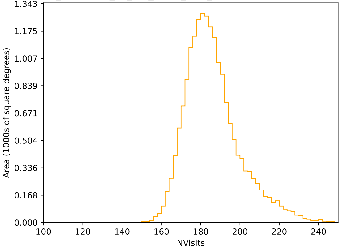
too_combined_no_nss_s10.0_v3.4_10yrs WFD r band: NVisits
