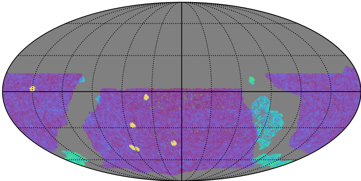
too_combined_no_nss_s10.0_v3.4_10yrs WFD g band: NVisits
