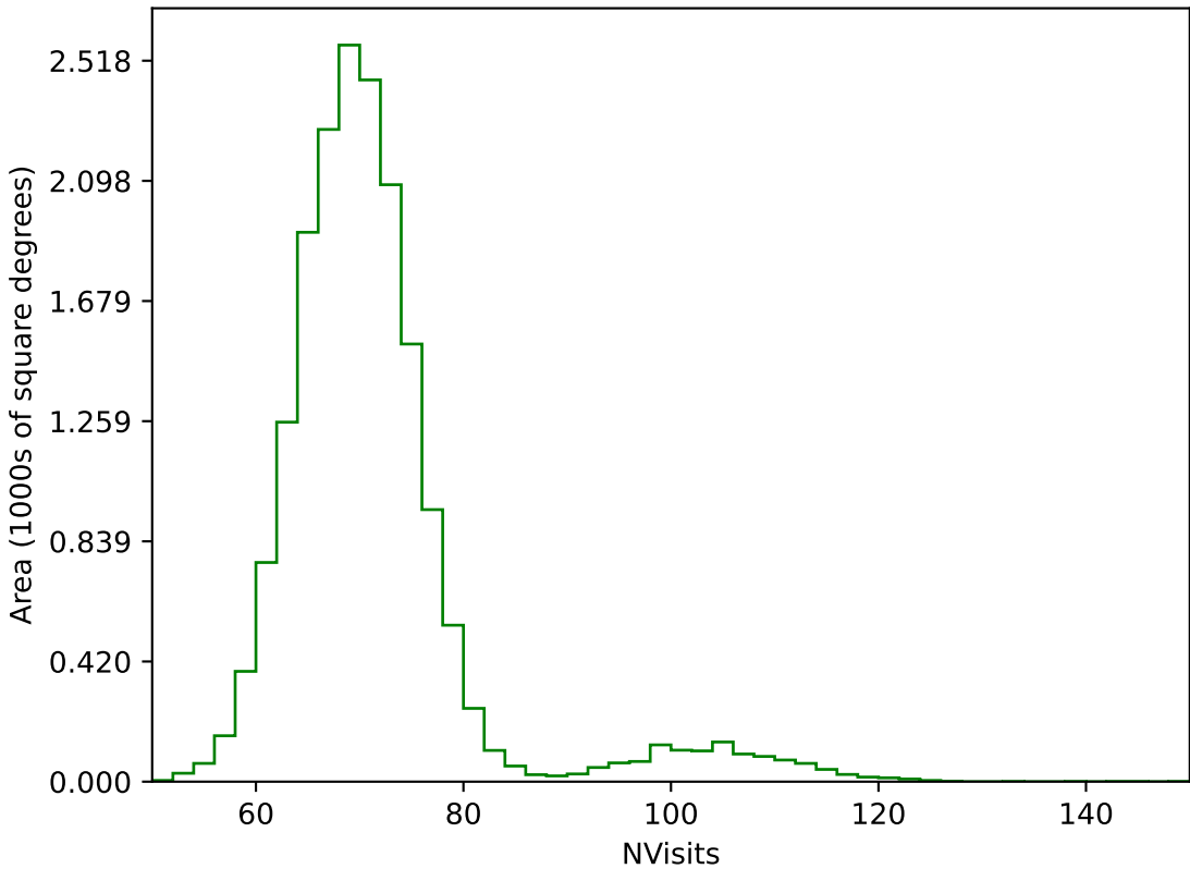
too_combined_no_nss_s10.0_v3.4_10yrs WFD g band: NVisits
