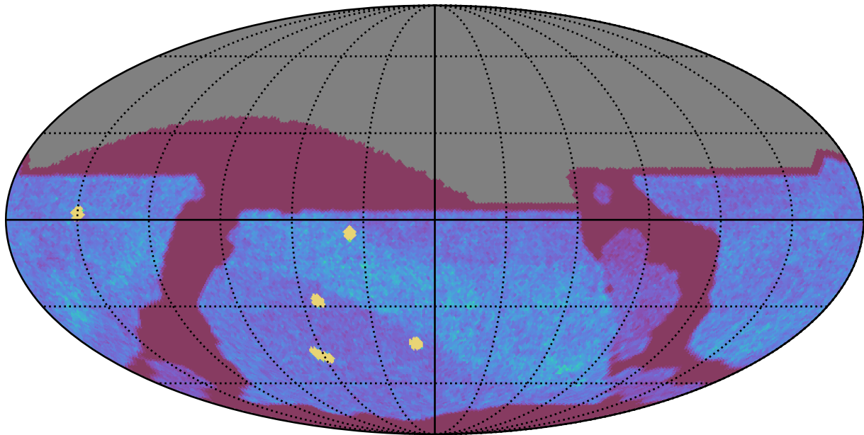
too_combined_no_nss_s10.0_v3.4_10yrs All sky z band: NVisits
