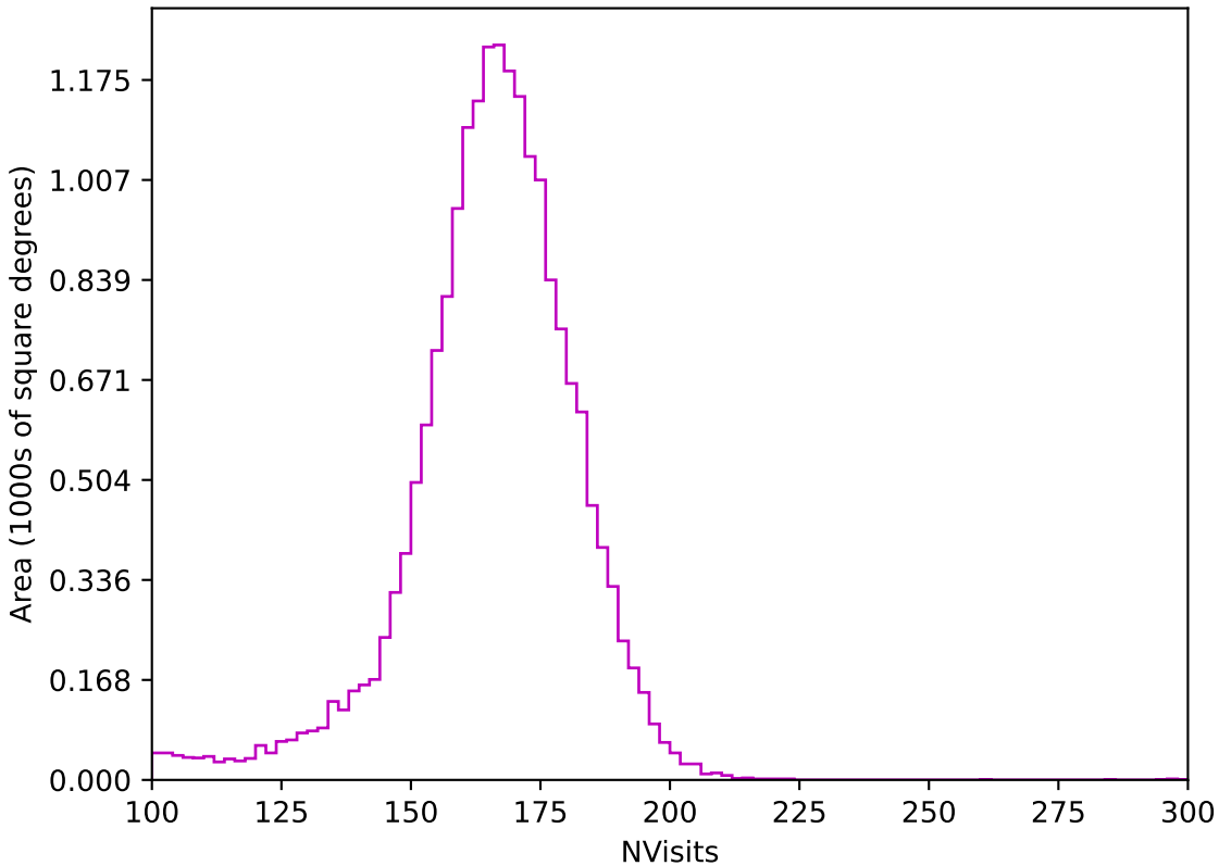
too_combined_no_nss_s10.0_v3.4_10yrs All sky z band: NVisits
