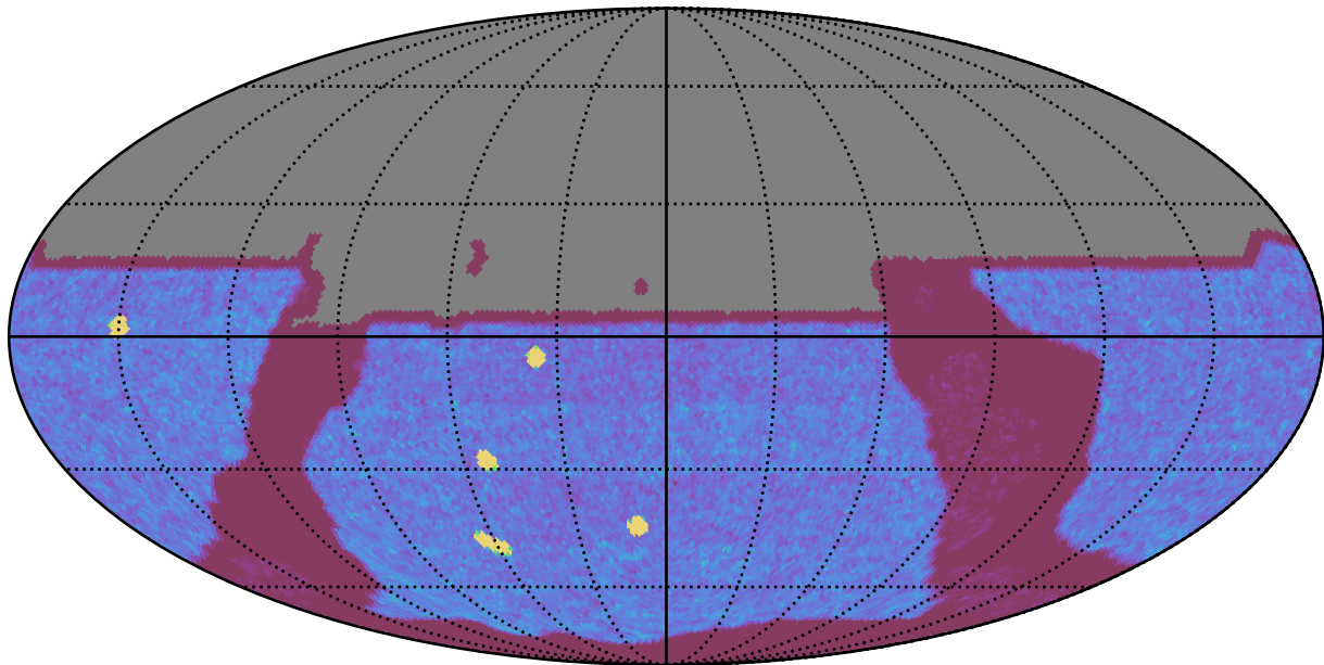
too_combined_no_nss_s10.0_v3.4_10yrs All sky y band: NVisits
