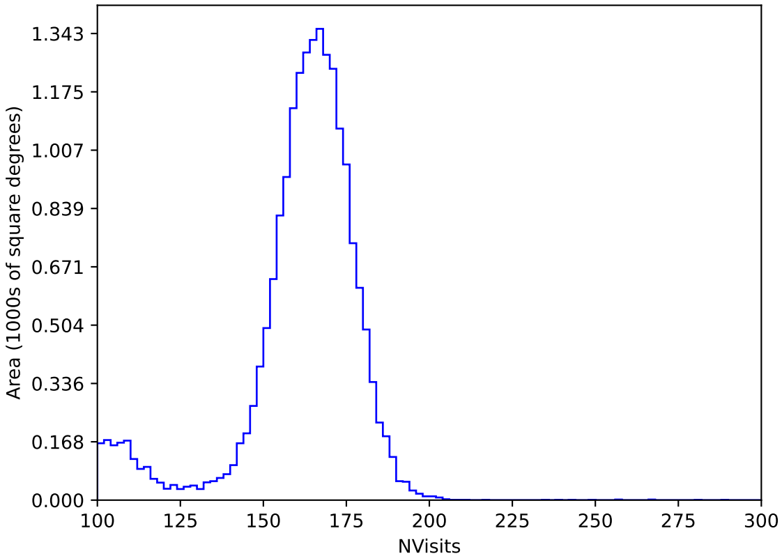
too_combined_no_nss_s10.0_v3.4_10yrs All sky y band: NVisits
