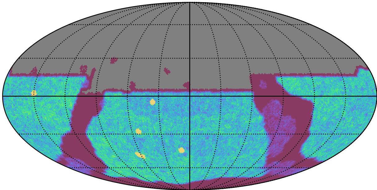
too_combined_no_nss_s10.0_v3.4_10yrs All sky u band: NVisits
