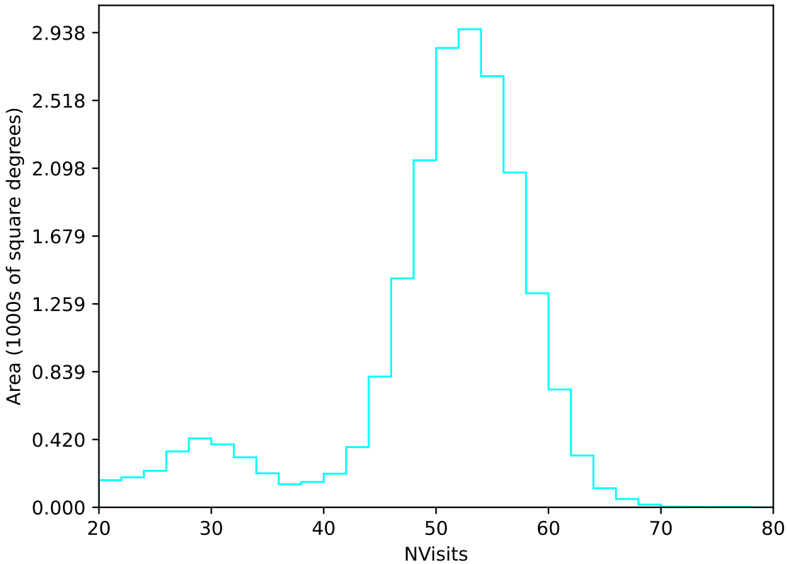
too_combined_no_nss_s10.0_v3.4_10yrs All sky u band: NVisits
