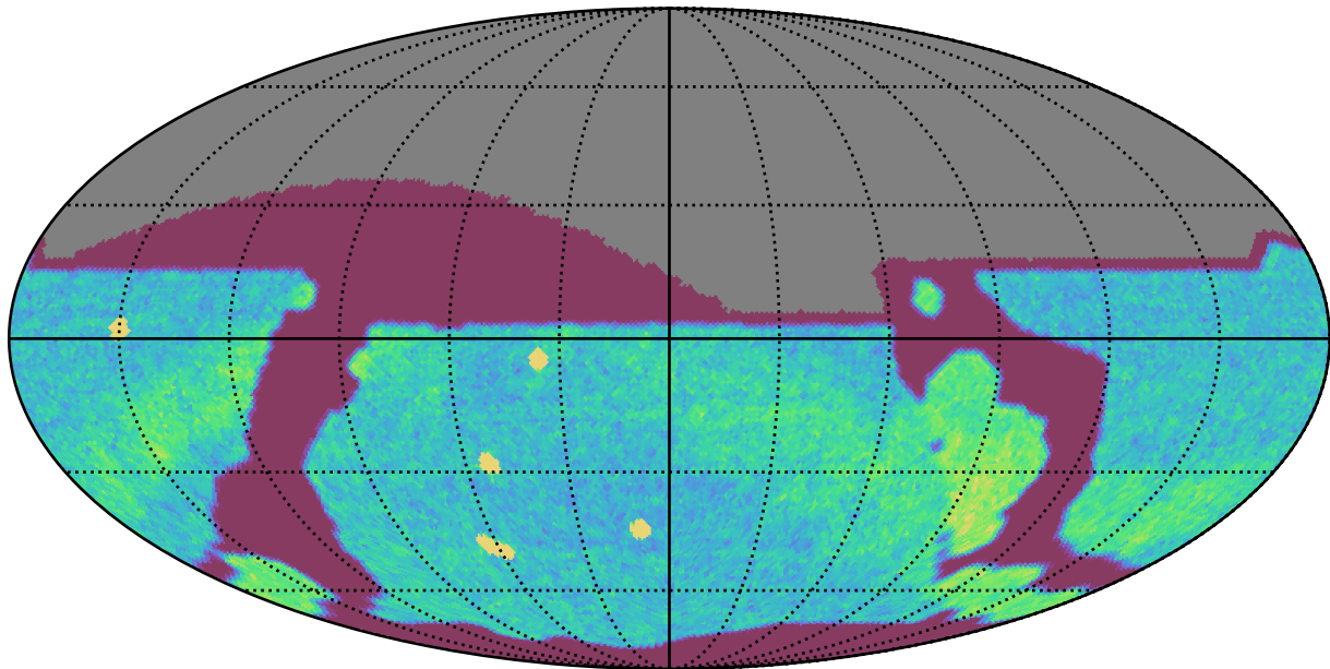
too_combined_no_nss_s10.0_v3.4_10yrs All sky r band: NVisits
