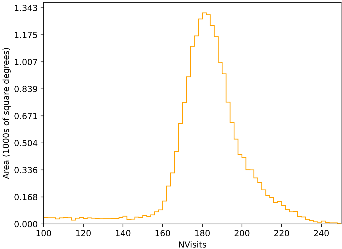
too_combined_no_nss_s10.0_v3.4_10yrs All sky r band: NVisits
