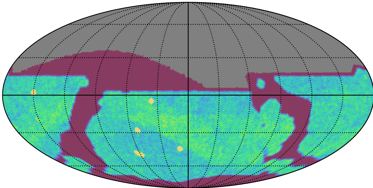
too_combined_no_nss_s10.0_v3.4_10yrs All sky i band: NVisits
