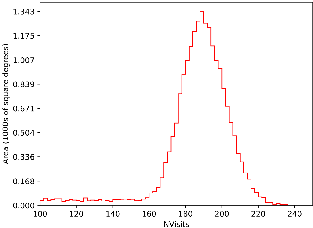
too_combined_no_nss_s10.0_v3.4_10yrs All sky i band: NVisits
