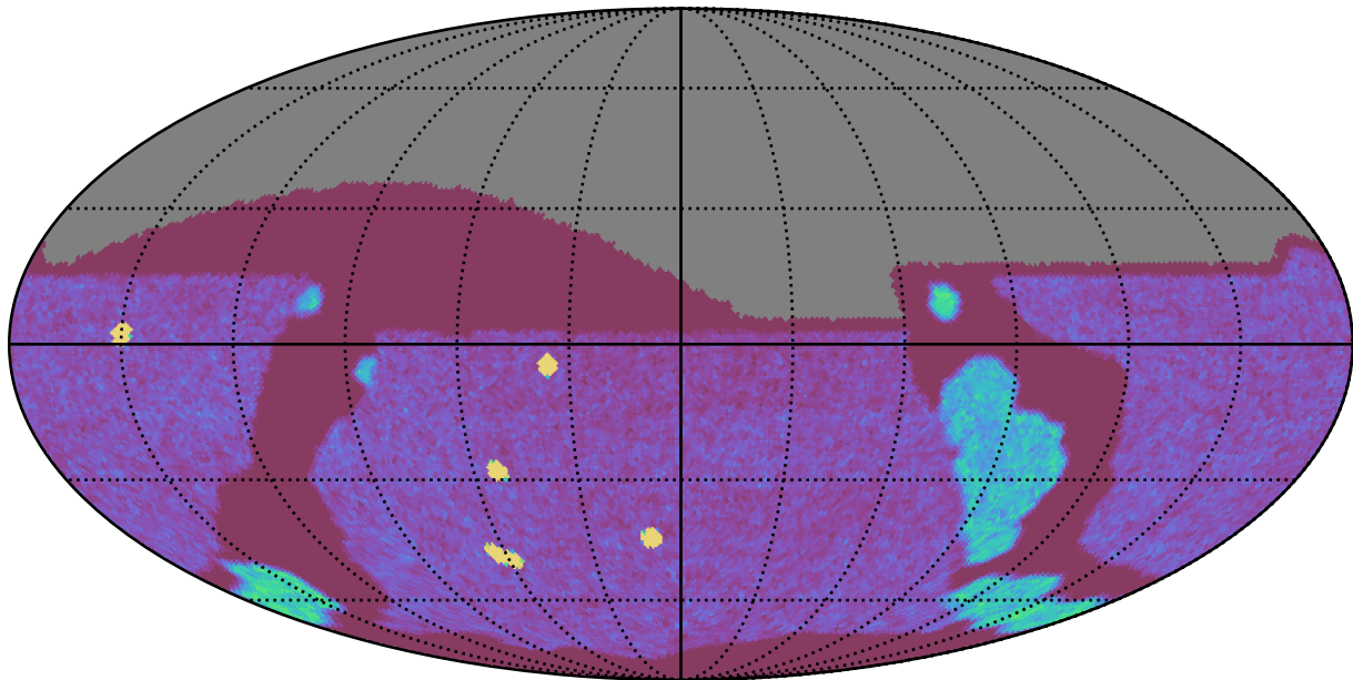
too_combined_no_nss_s10.0_v3.4_10yrs All sky g band: NVisits
