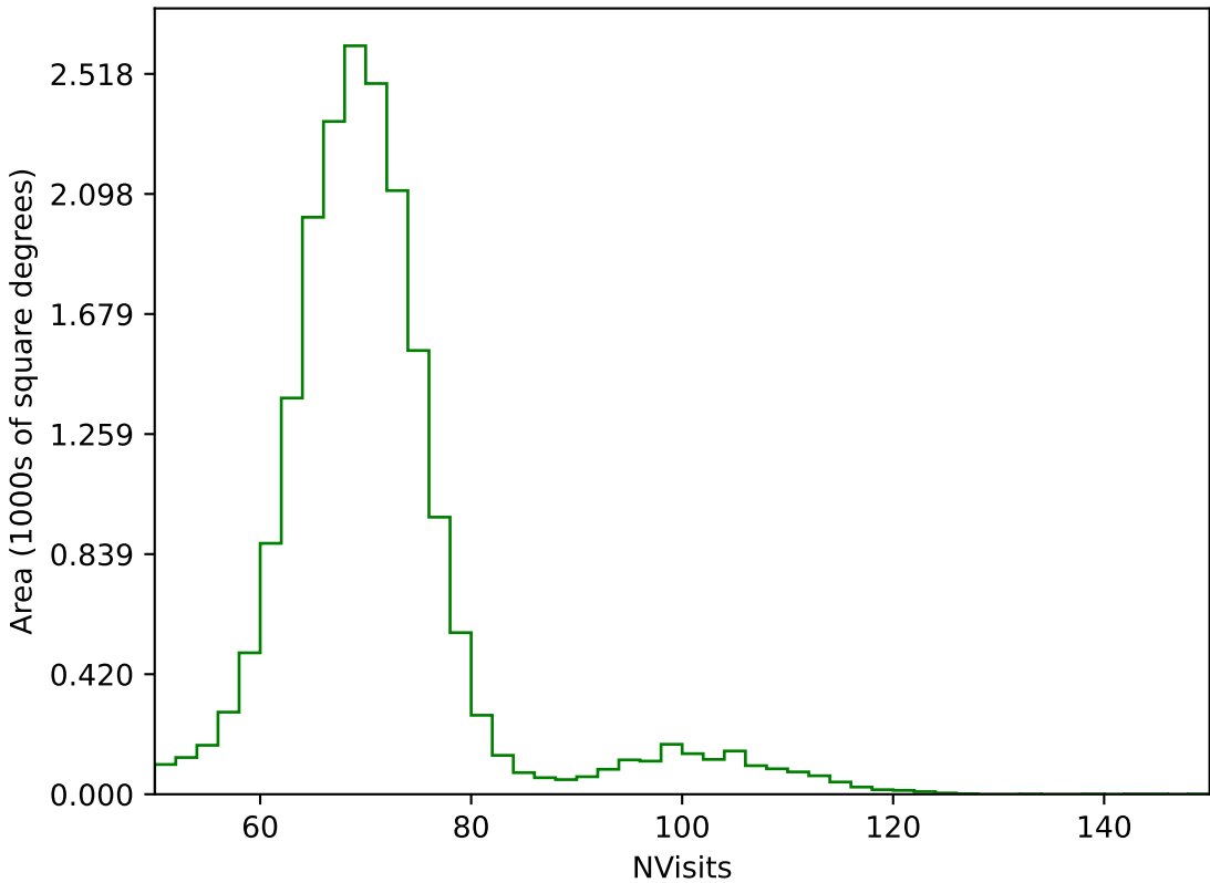
too_combined_no_nss_s10.0_v3.4_10yrs All sky g band: NVisits
