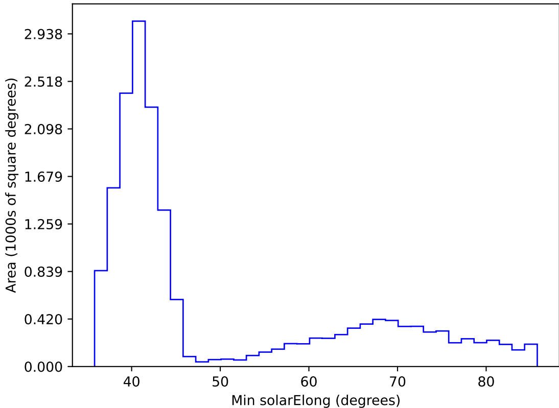
too_combined_no_nss_s10.0_v3.4_10yrs WFD i band: Min solarElong
