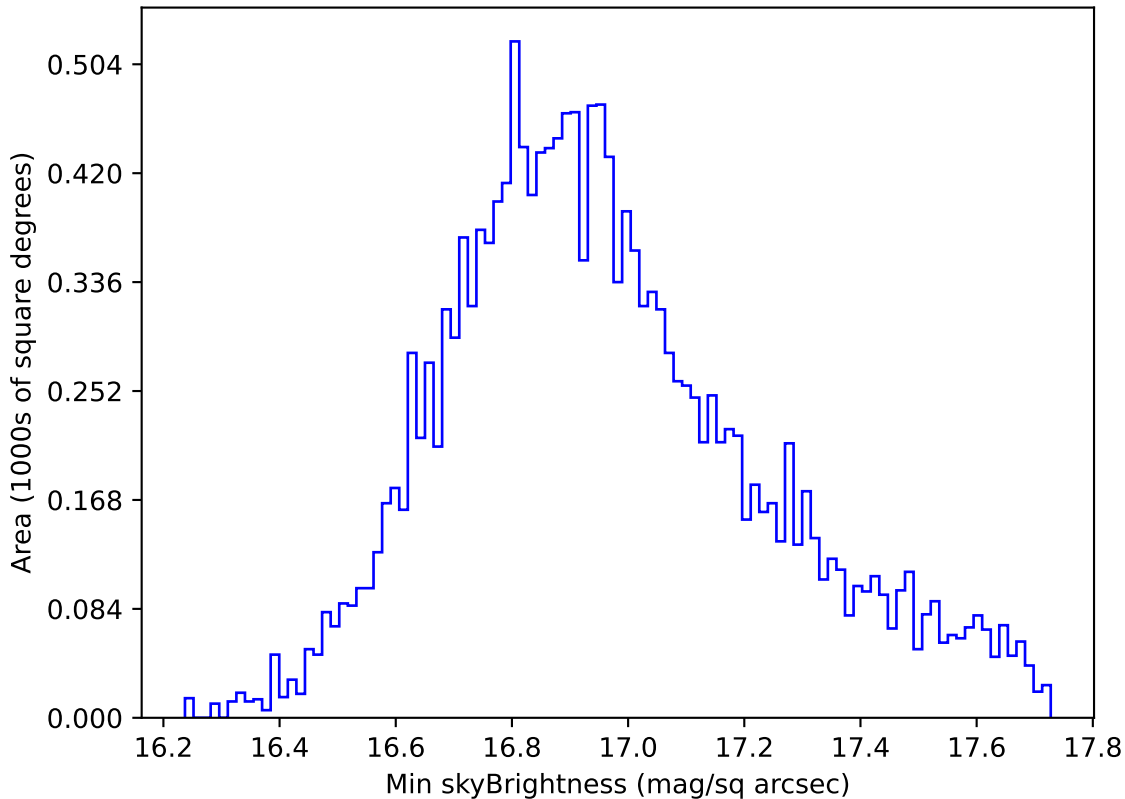
too_combined_no_nss_s10.0_v3.4_10yrs WFD all bands: Min skyBrightness
