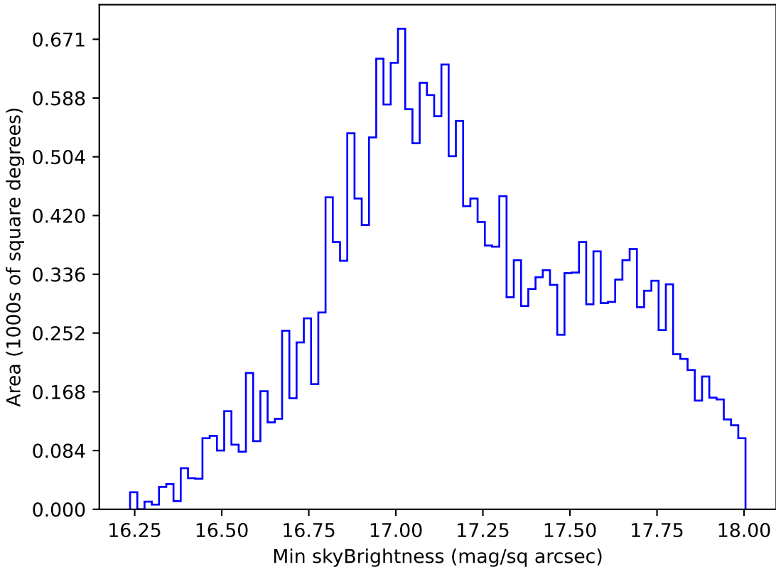
too_combined_no_nss_s10.0_v3.4_10yrs All sky y band: Min skyBrightness
