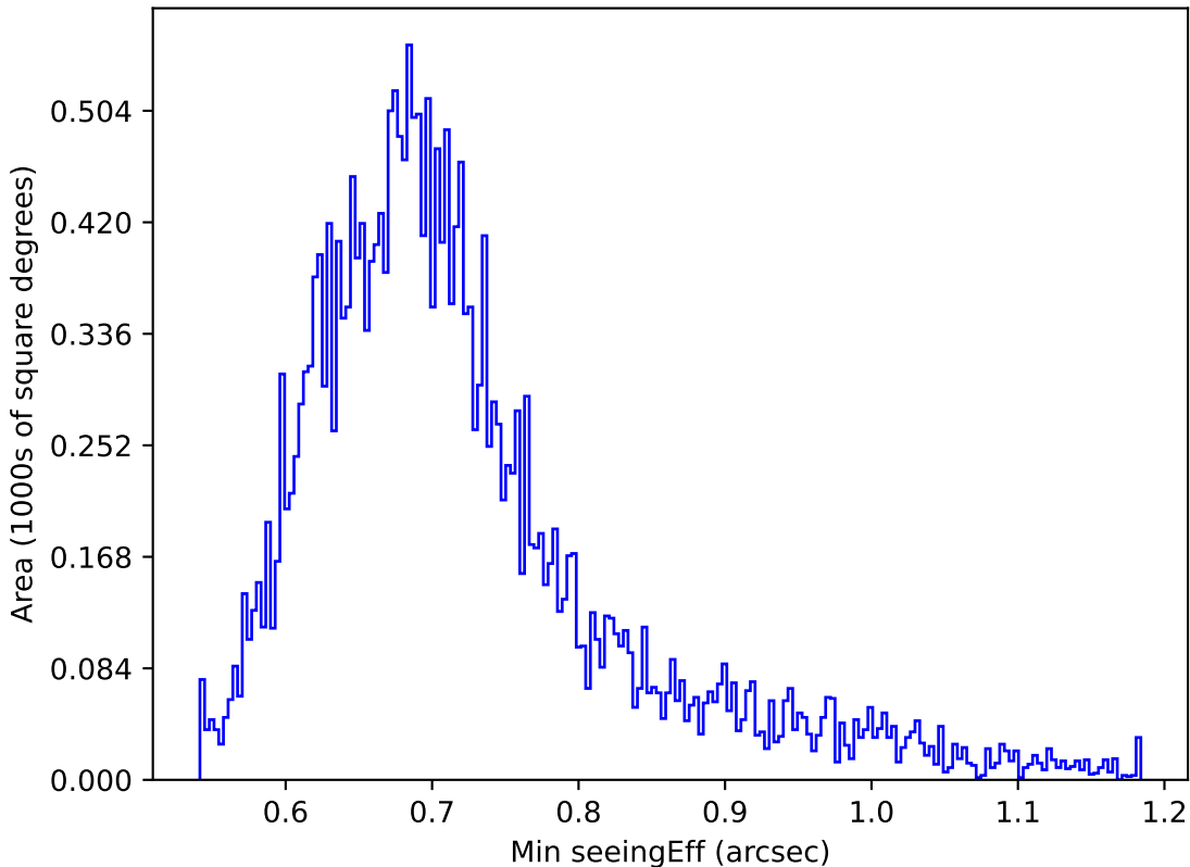
too_combined_no_nss_s10.0_v3.4_10yrs Yr 1 z band: Min seeingEff
