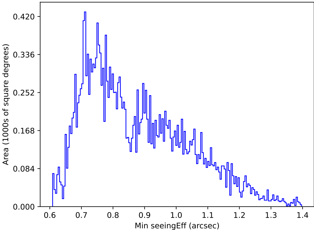
too_combined_no_nss_s10.0_v3.4_10yrs Yr 1 u band: Min seeingEff
