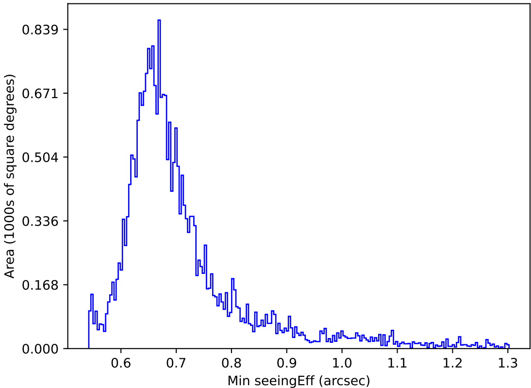
too_combined_no_nss_s10.0_v3.4_10yrs Yr 1 i band: Min seeingEff
