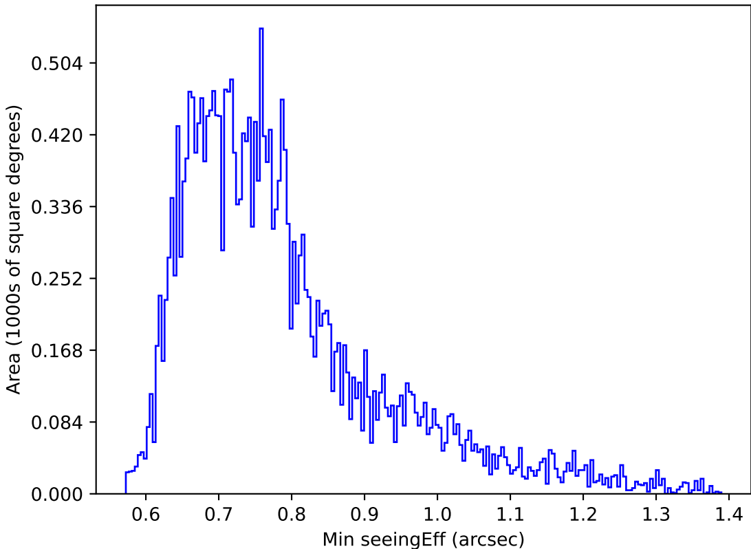
too_combined_no_nss_s10.0_v3.4_10yrs Yr 1 g band: Min seeingEff
