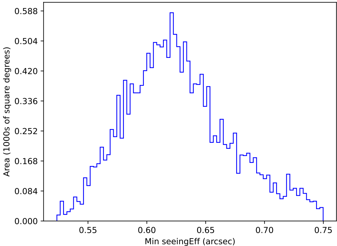
too_combined_no_nss_s10.0_v3.4_10yrs WFD y band: Min seeingEff
