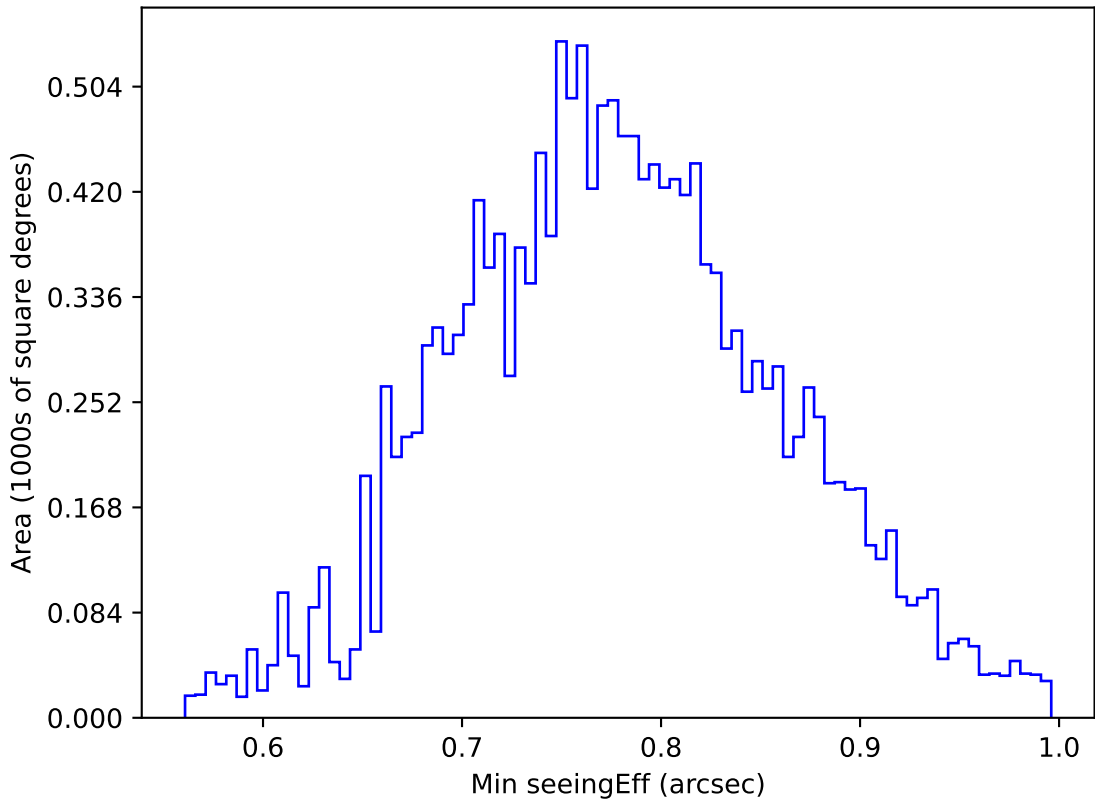
too_combined_no_nss_s10.0_v3.4_10yrs WFD u band: Min seeingEff
