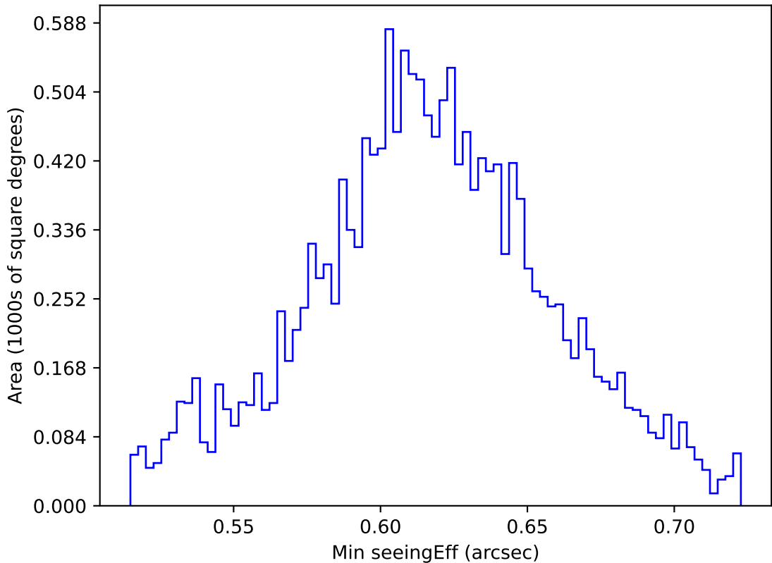
too_combined_no_nss_s10.0_v3.4_10yrs WFD r band: Min seeingEff
