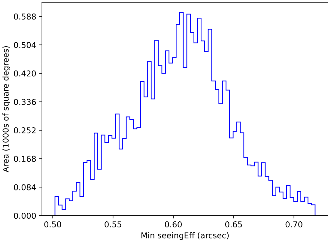
too_combined_no_nss_s10.0_v3.4_10yrs WFD i band: Min seeingEff
