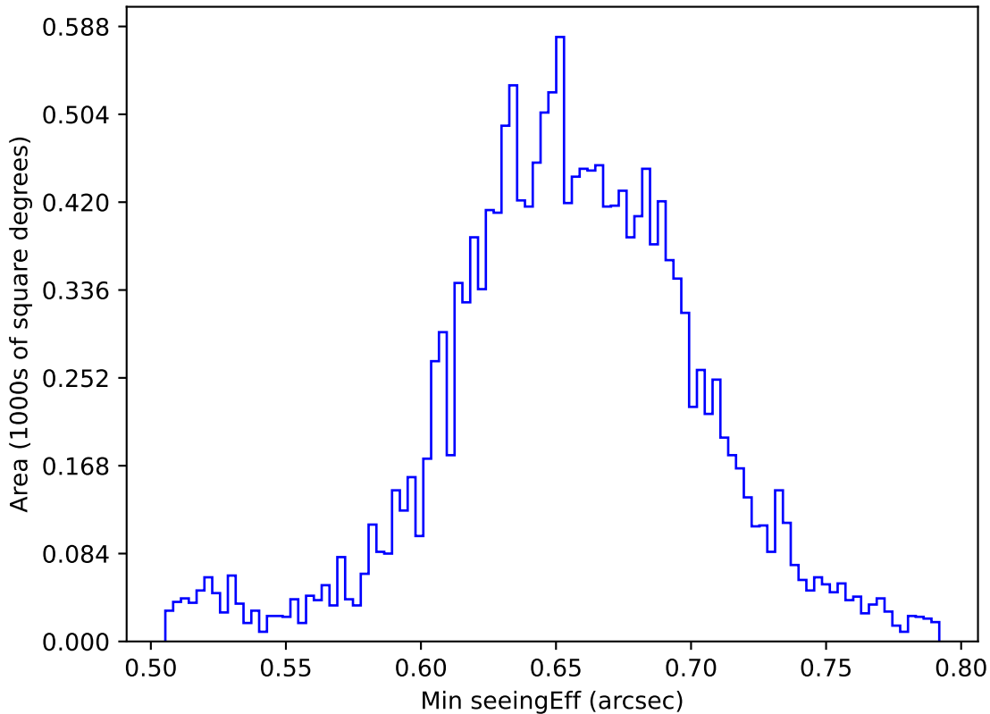
too_combined_no_nss_s10.0_v3.4_10yrs WFD g band: Min seeingEff
