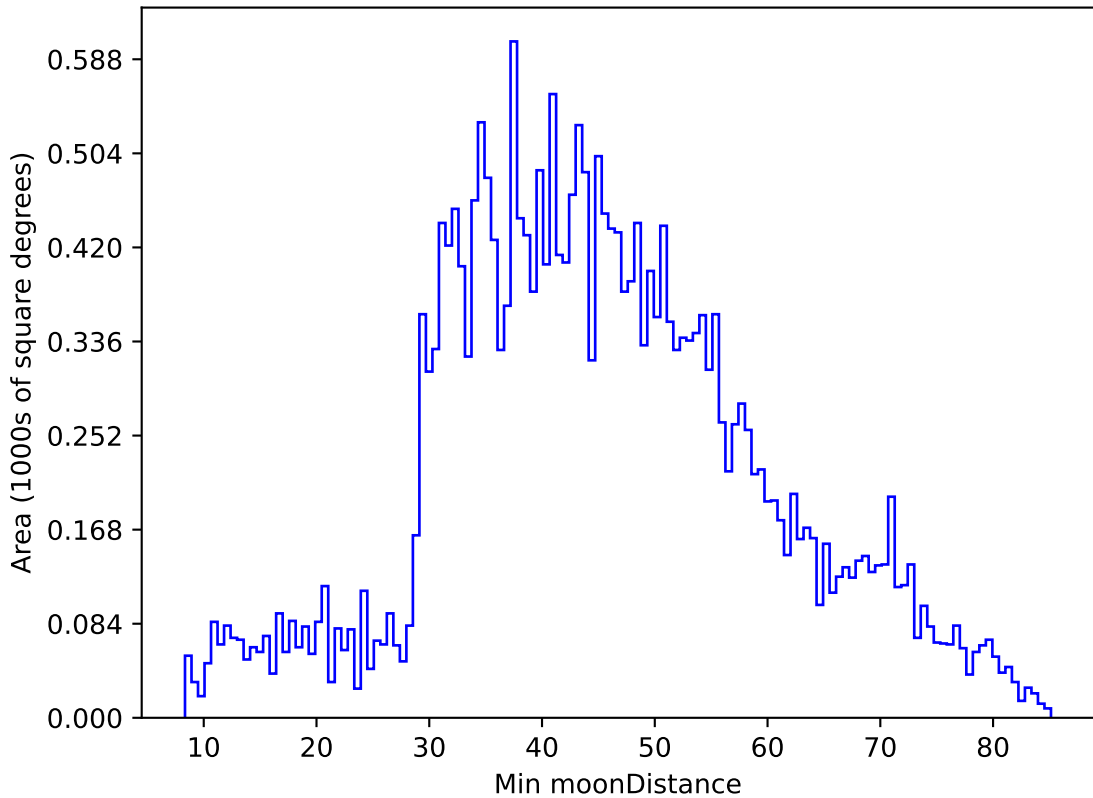
too_combined_no_nss_s10.0_v3.4_10yrs All sky g band: Min moonDistance
