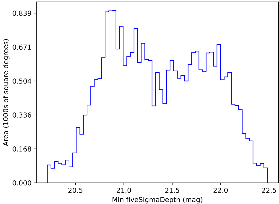
too_combined_no_nss_s10.0_v3.4_10yrs All sky z band: Min fiveSigmaDepth
