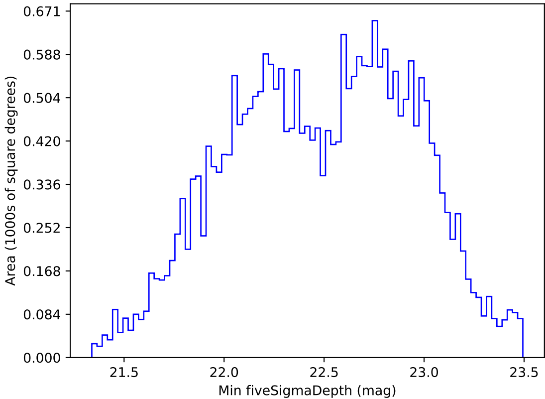
too_combined_no_nss_s10.0_v3.4_10yrs All sky r band: Min fiveSigmaDepth
