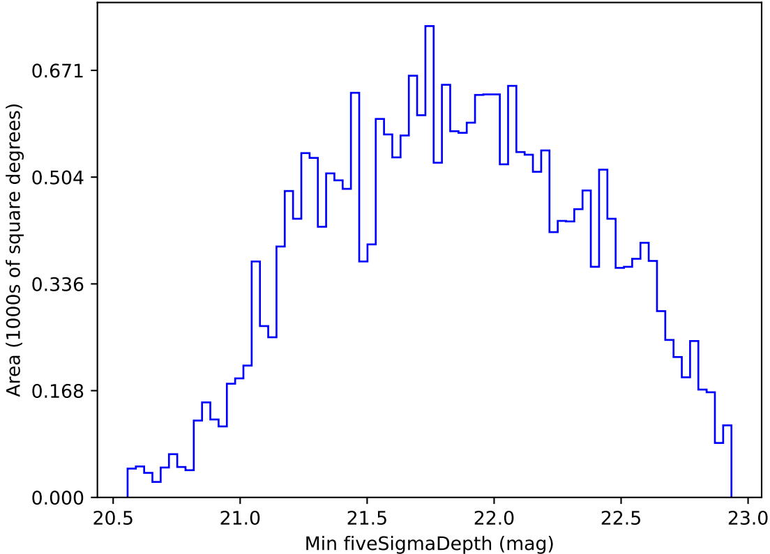
too_combined_no_nss_s10.0_v3.4_10yrs All sky i band: Min fiveSigmaDepth
