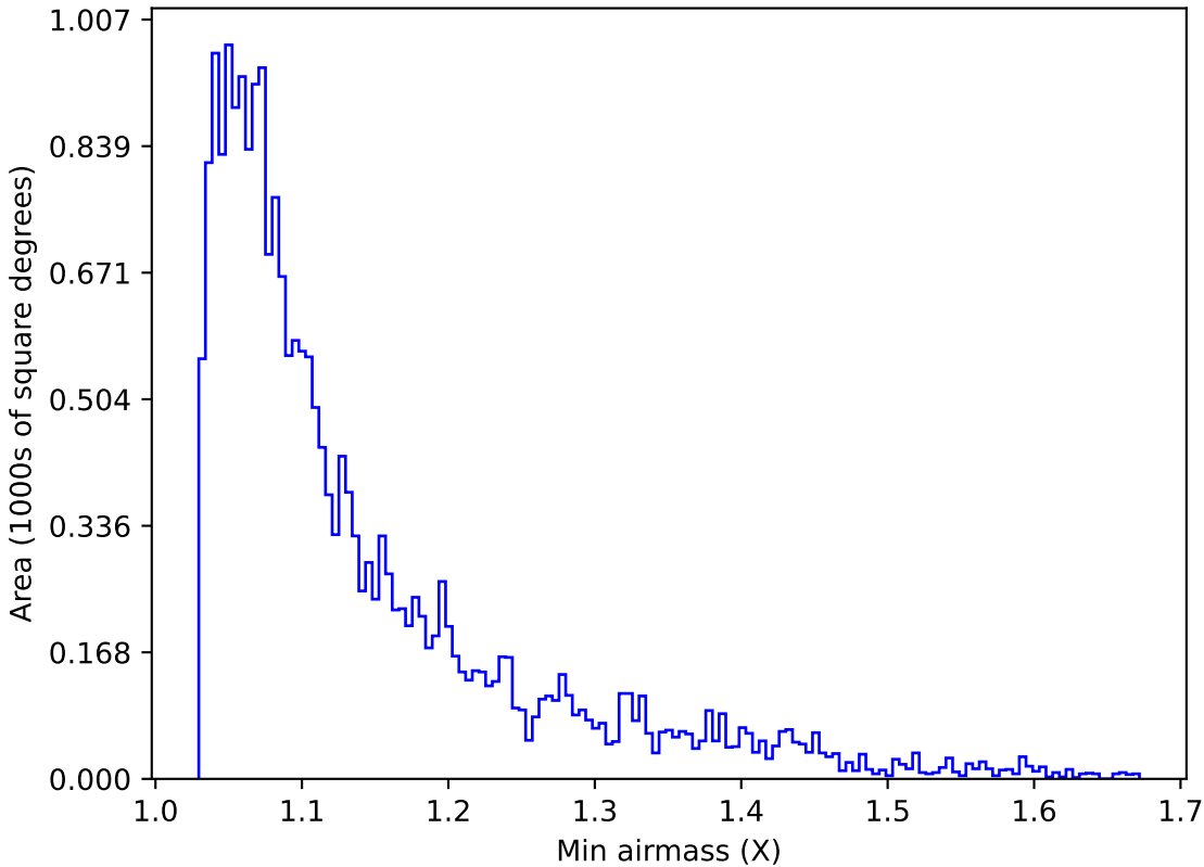
too_combined_no_nss_s10.0_v3.4_10yrs Yr 1 u band: Min airmass
